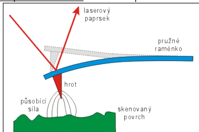
Fig. Schema of the Atomic force microscope.
