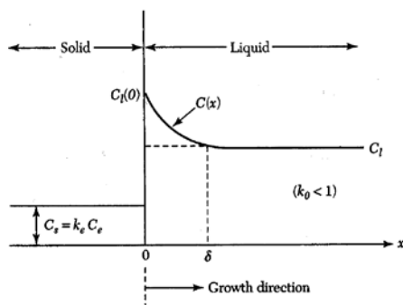
Doping distribution near the solid-melt interface.
