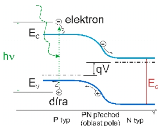
P-N junction- energy bands
