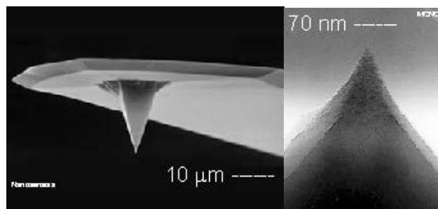
Fig. Cantilever.
