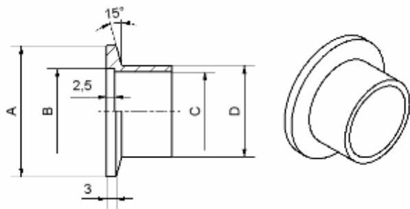
Flanges with tabulation, Centering Rings
