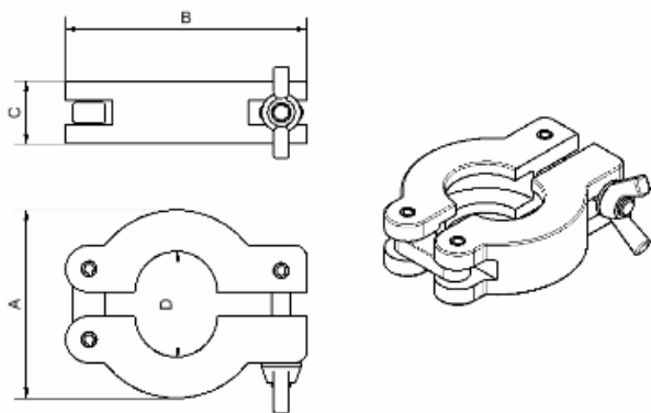
Clamping Ring
