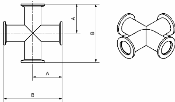
4-way cross
