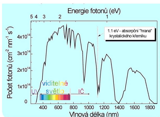
Solar spectrum after passing through the atmosphere
