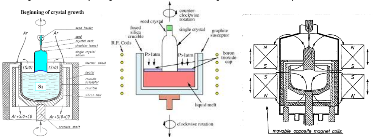
Fig.4. Czochralski growth of Si, LEC CZ growth of GaAs, Mixing of the melt by Eddy currents
