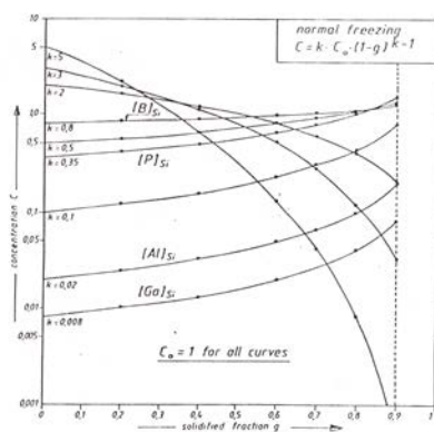
Fig. 7. Distribution of the impurity concentration in silicon.
