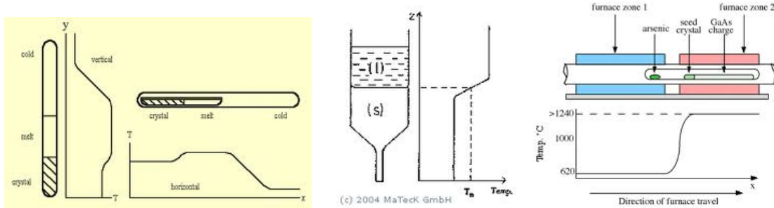
Fig.8. Bridgman method
