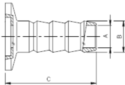
Flange with Hose nozzle, Flexible Bellows with Flanges
