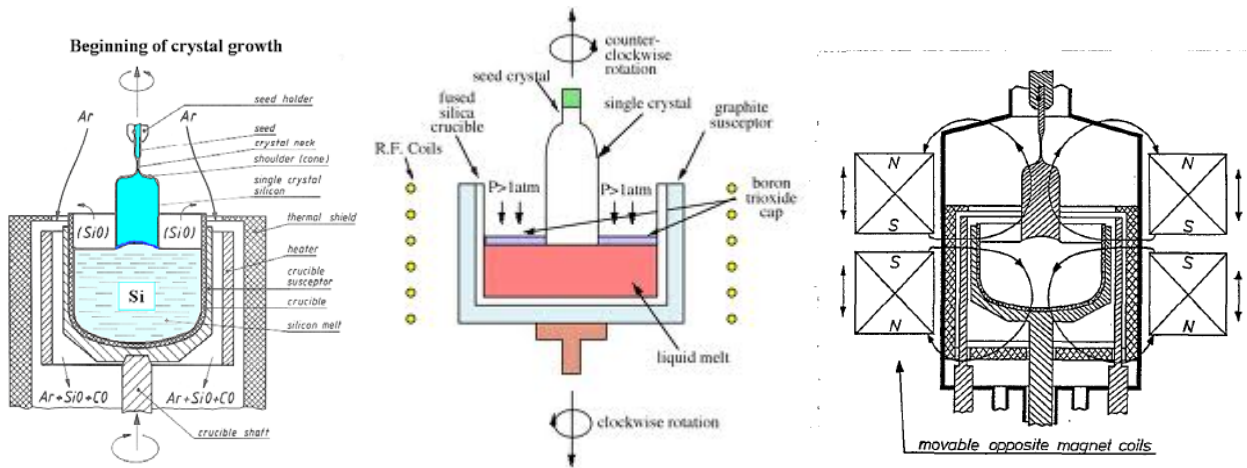
Obr.13. Czochralski method - a) Si growth, b) Liquid Encapsulated Czochralski - LEC CZ (Growth of GaAs, CdTe, InP...) – Boron trioxide ( B_2O_3 ) cap is used to prevent melt decomposition due to the leak of the more volatile component and to form a separating layer between crucible and charge. c) Using nonstationary magnetic field for melt mixing – Foucault's eddy currents.
