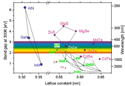
Fig.2. Classification of semiconductors according to the position in the periodic table, to the width of the forbidden gap and to the lattice constant, respectively.
