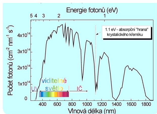
Solar spectrum after passing through the
