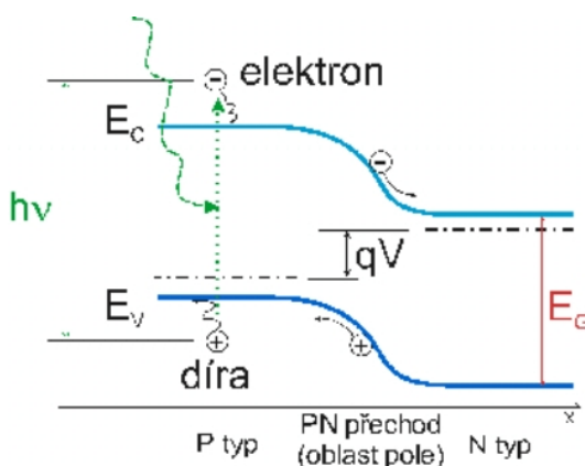
P-N junction- energy bands atmosphere
