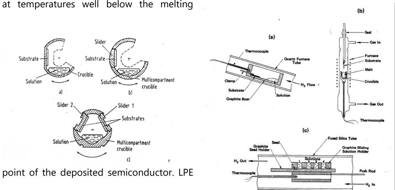
Fig. 5. Drawings of LPE systems: (a) tipper system after Nelson, (1963); (b) dipper system after Rupprecht, (1967) and (c) slider system after Panish, et al. (1969).
