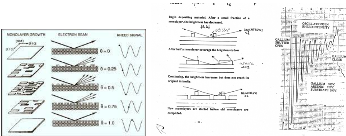
Fig.10. RHEED method- Reflection High Energy Electron Diffraction
