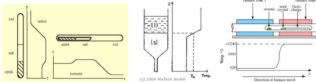
Fig.8. Bridgman method
