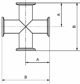
4-way cross
