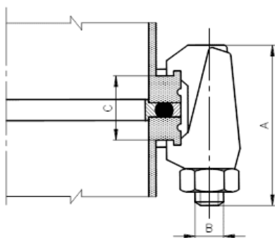
Flange with Hose nozzle, Flexible Bellows with Flanges
