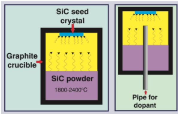
Fig.11 Scheme of the PVT sublimation apparatus. Inserting a tube allows various dopants and other gases affecting SiC growth to be delivered on the substrate.
