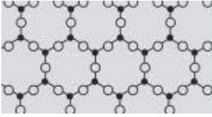
Crystalline SiO 2 Quartz glass – amorphous SiO 2
