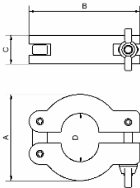
Clamping Ring
