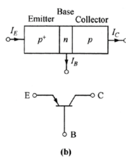
Symbols and nomenclatures of (a) n-p-n transistors and (b) p-n-p transistors.
