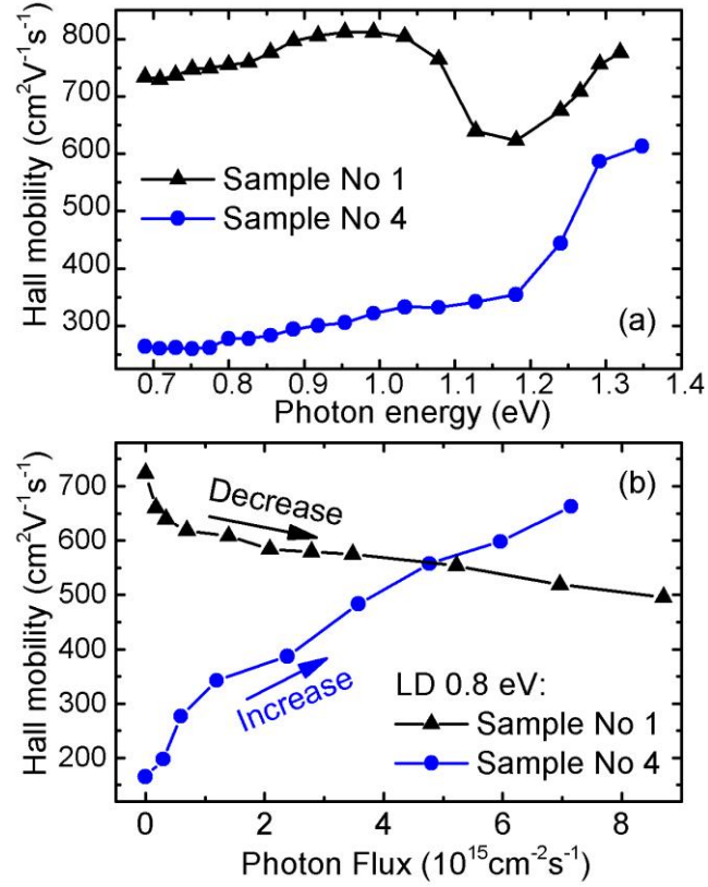
Fig. 4.6. Hall mobility spectra (a) and Hall mobility versus photon flux (b) at 0.8 eV photon energy measured in samples No 1 (unusual behavior) and No 4 (common behavior).
