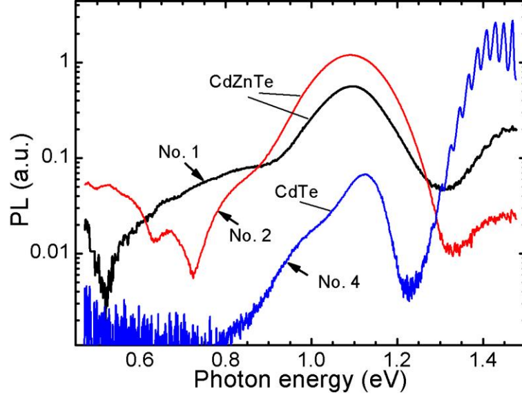
Fig. 4.4. PL spectra representing DLs transitions in CdZnTe and CdTe n -type samples. Affiliation of each curve is labeled by a number from the Table 4.
