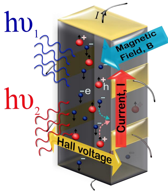
Fig. 3.3. Basic principles of DWPHEs measurements.
