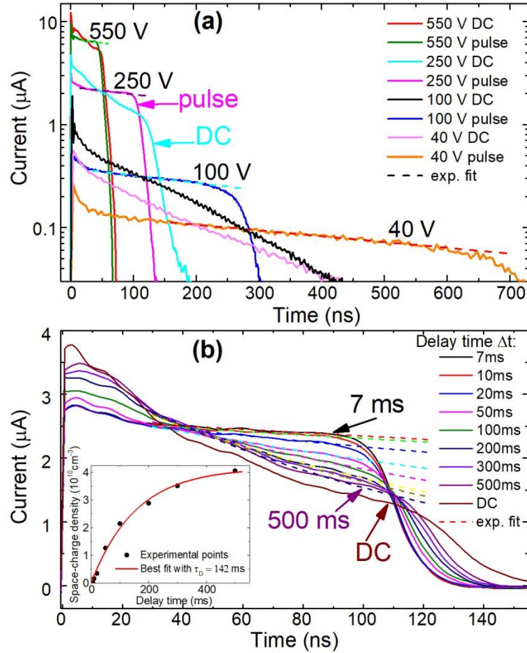
Fig. 6.1. (a) L-TCT CWFs measured at 40V, 100 V, 250 V and 550 V bias in the pulse with \Delta t=10\text{ms} and steady-state (DC) regimes corresponding to the flat/tilted CWFs. (b) L-TCT CWFs measured at 250 V bias in the pulse mode. Each waveform was obtained with given delay time \Delta t . Dashed lines plot the exponential fit of transients. The inset shows the space-charge density as a function of the delay time according to Eq. (2.40).
